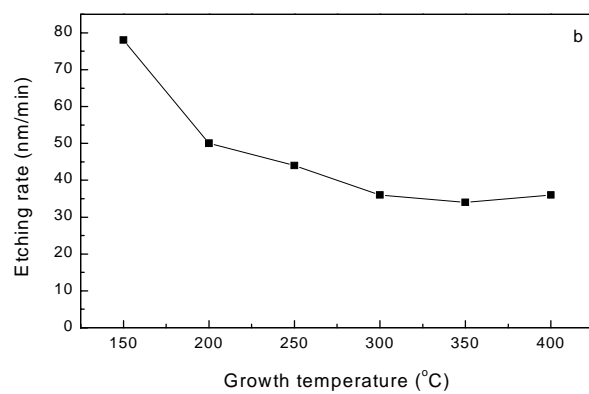
Figure 13. The etching rate for Al 2 O 3 films at 60 °C. The etching solution was (a) 7 M H 3 PO 4 and (b) 0.1 M NaOH.
