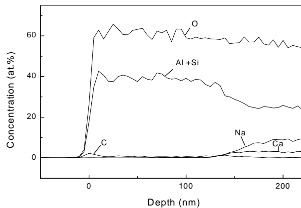
Figure 11. Element depth profiles of an \text{Al}_2\text{O}_3 film deposited at 150 \text{ }^\circ\text{C} as analysed by TOF-ERDA.
